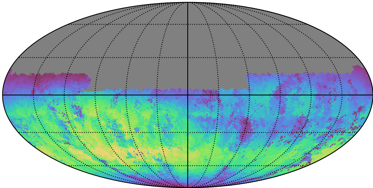
noroll_mjdp270_v3.4_10yrs Yr 1 u band: Median skyBrightness
