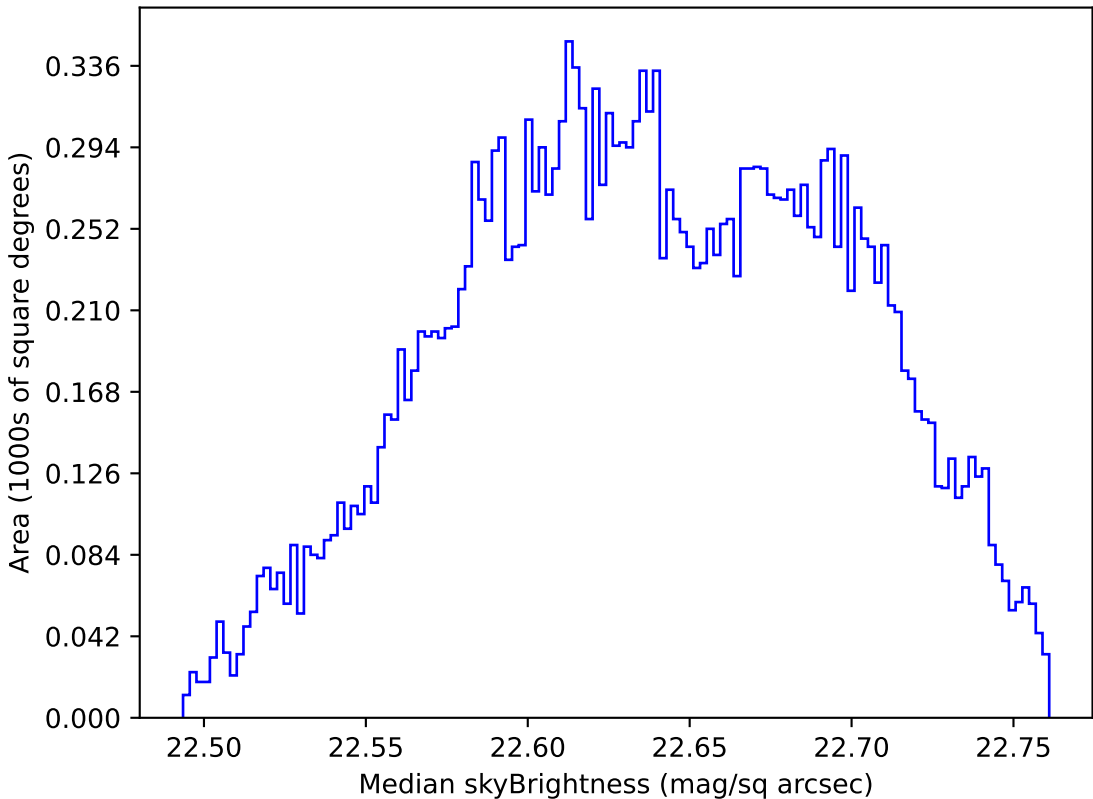
noroll_mjdp270_v3.4_10yrs Yr 1 u band: Median skyBrightness
