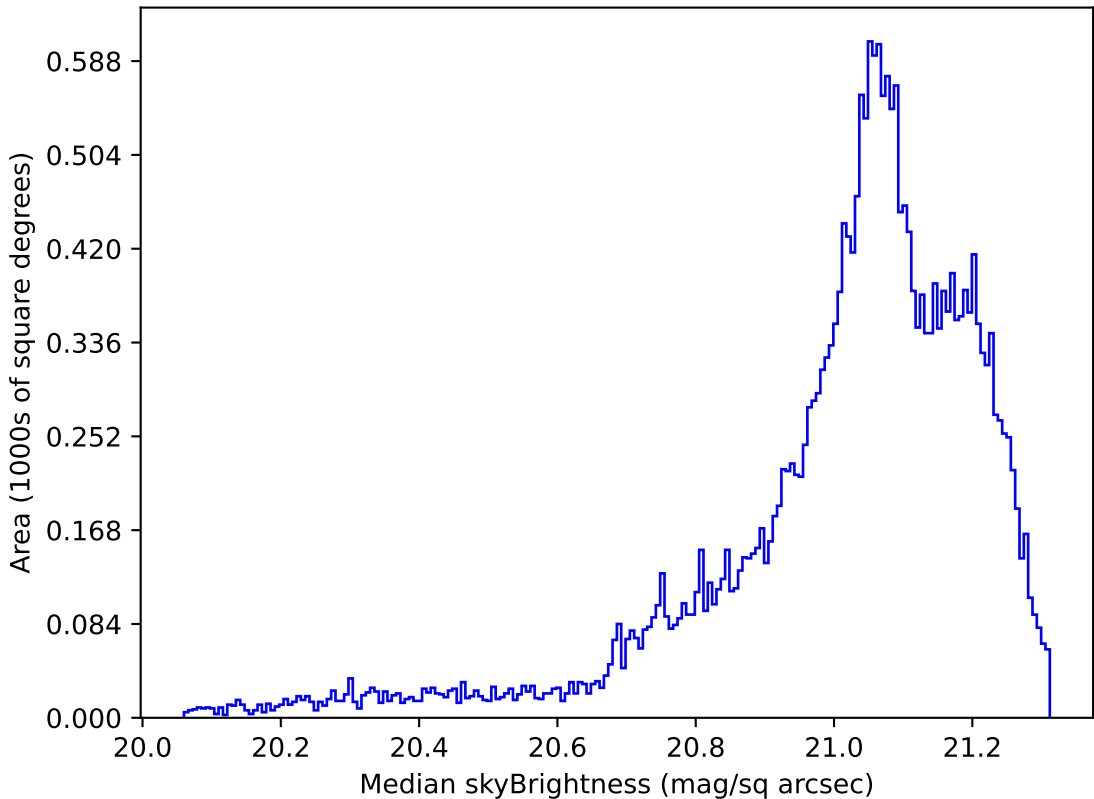
noroll_mjdp270_v3.4_10yrs Yr 1 r band: Median skyBrightness
