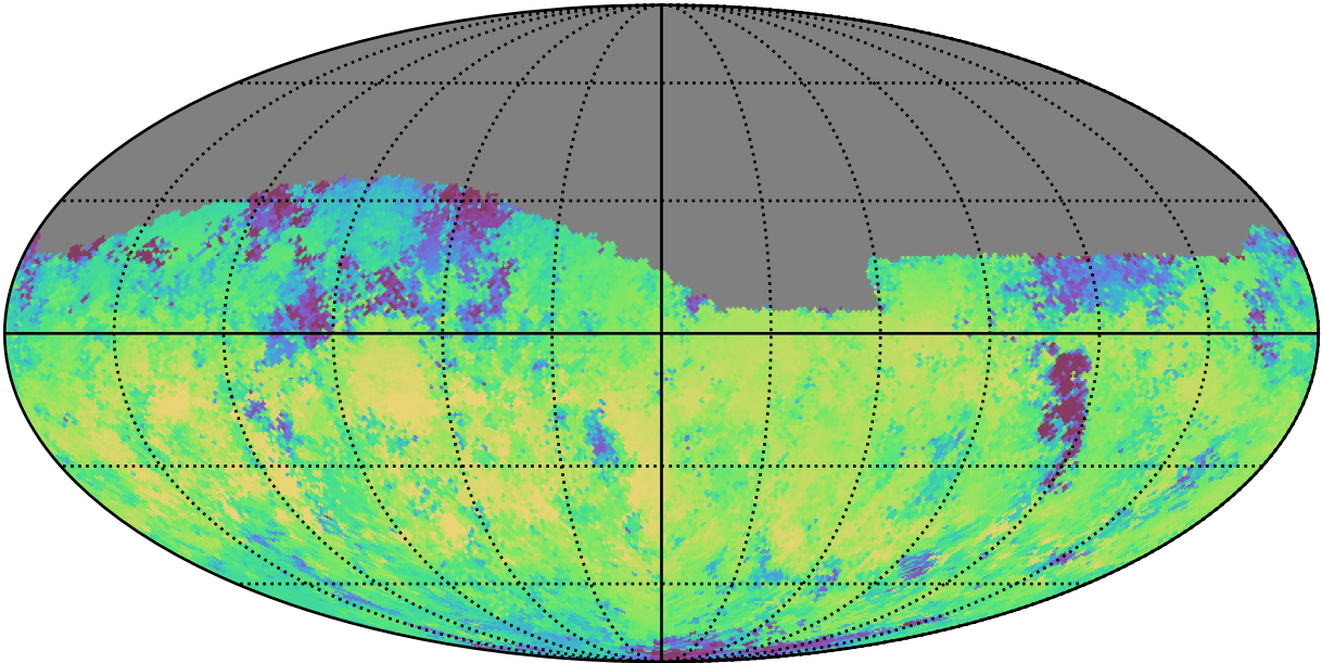
noroll_mjdp270_v3.4_10yrs Yr 1 i band: Median skyBrightness
