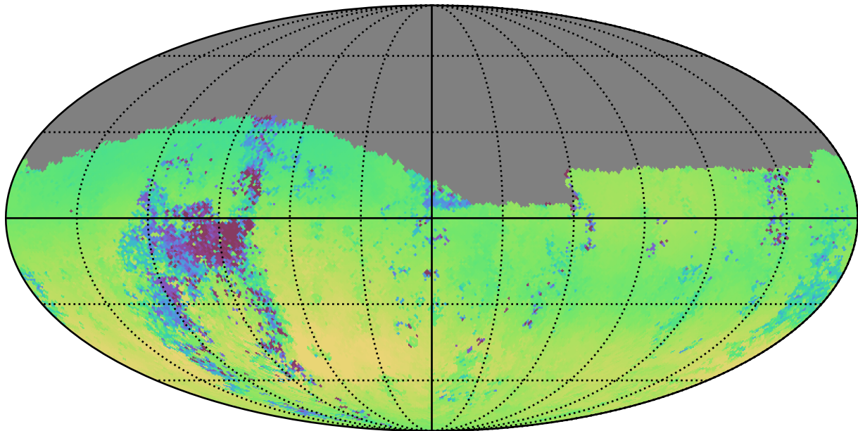
noroll_mjdp270_v3.4_10yrs Yr 1 g band: Median skyBrightness
