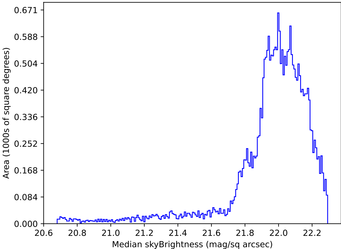
noroll_mjdp270_v3.4_10yrs Yr 1 g band: Median skyBrightness
