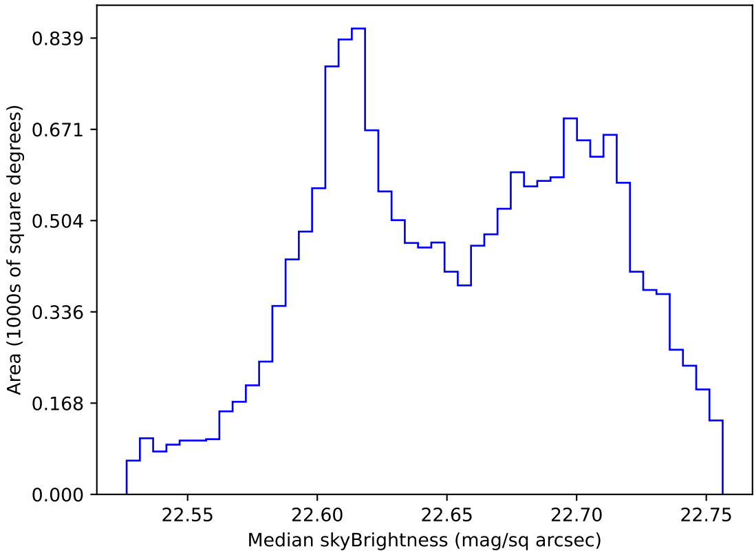
noroll_mjdp270_v3.4_10yrs WFD u band: Median skyBrightness
