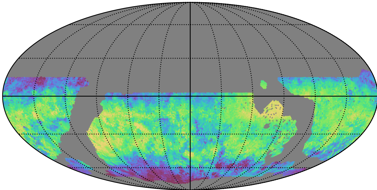
noroll_mjdp270_v3.4_10yrs WFD i band: Median skyBrightness
