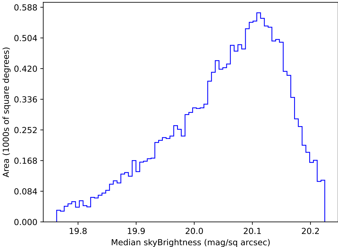
noroll_mjdp270_v3.4_10yrs WFD i band: Median skyBrightness
