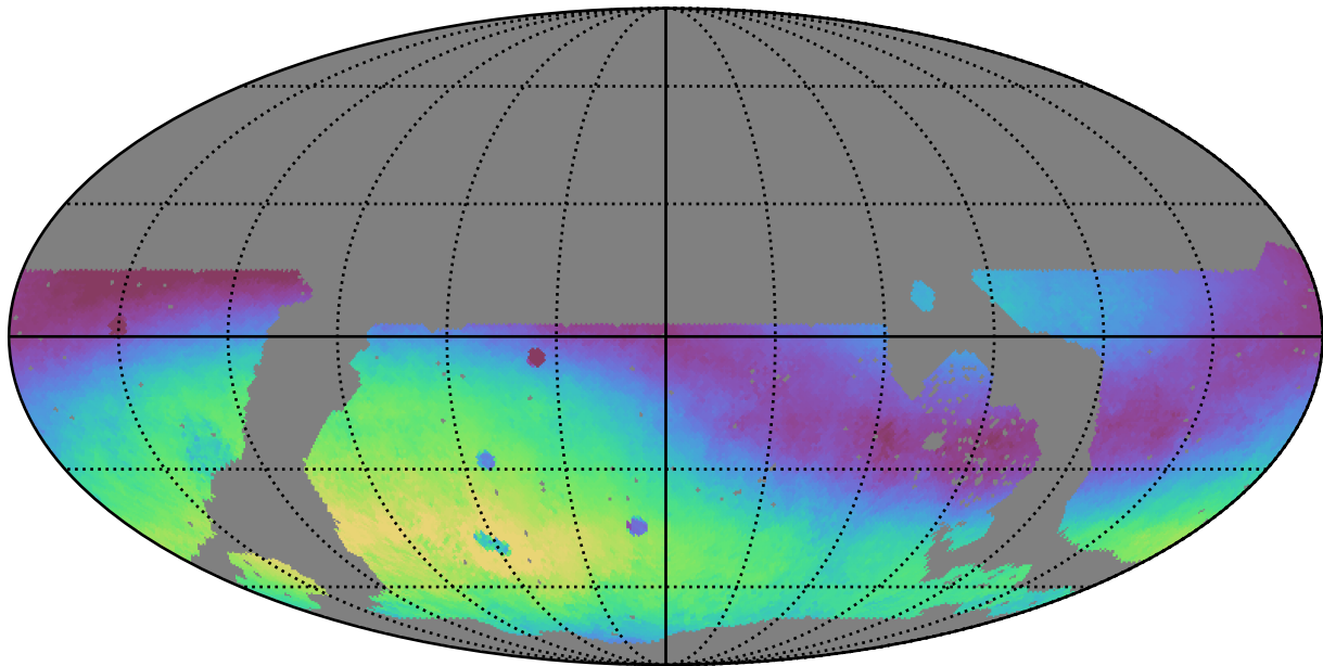
noroll_mjdp270_v3.4_10yrs WFD g band: Median skyBrightness
