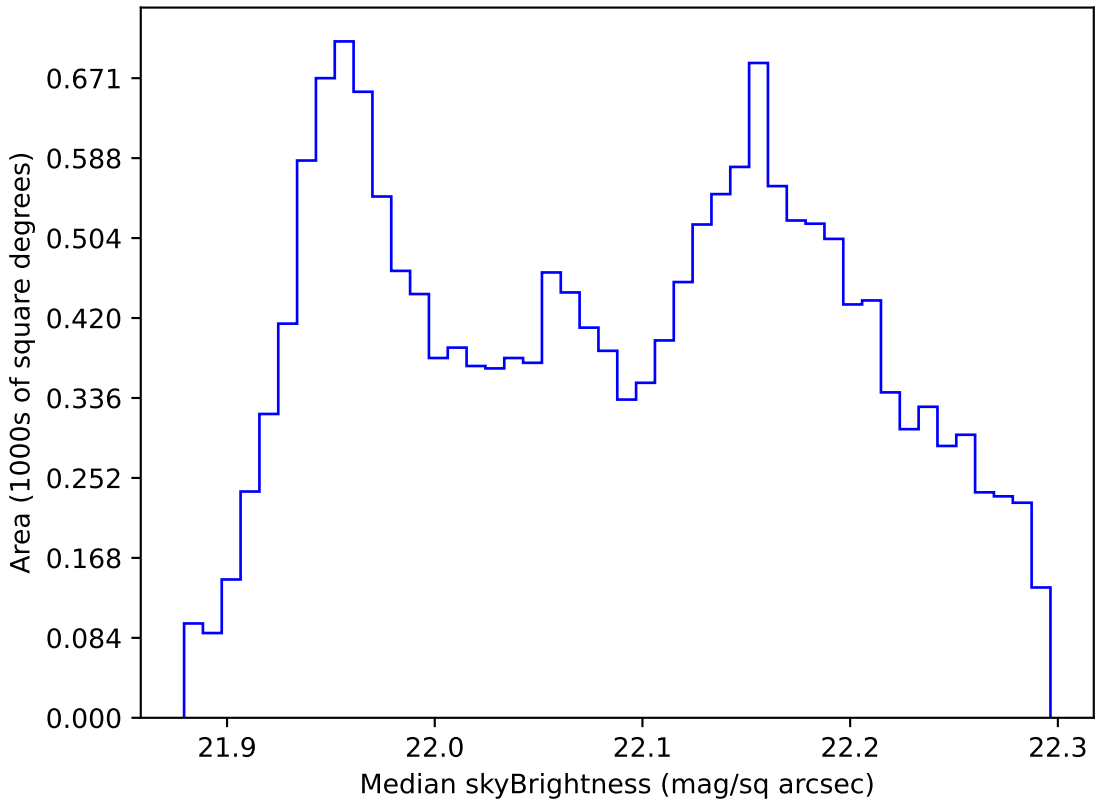
noroll_mjdp270_v3.4_10yrs WFD g band: Median skyBrightness
