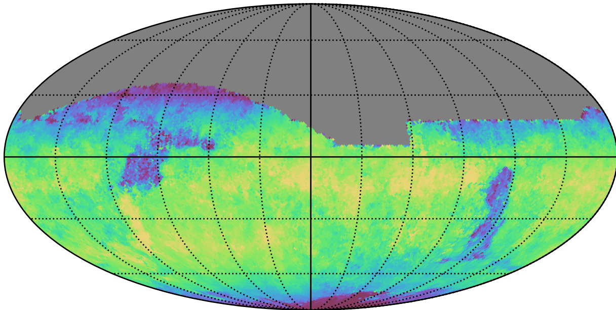
noroll_mjdp270_v3.4_10yrs All sky z band: Median skyBrightness
