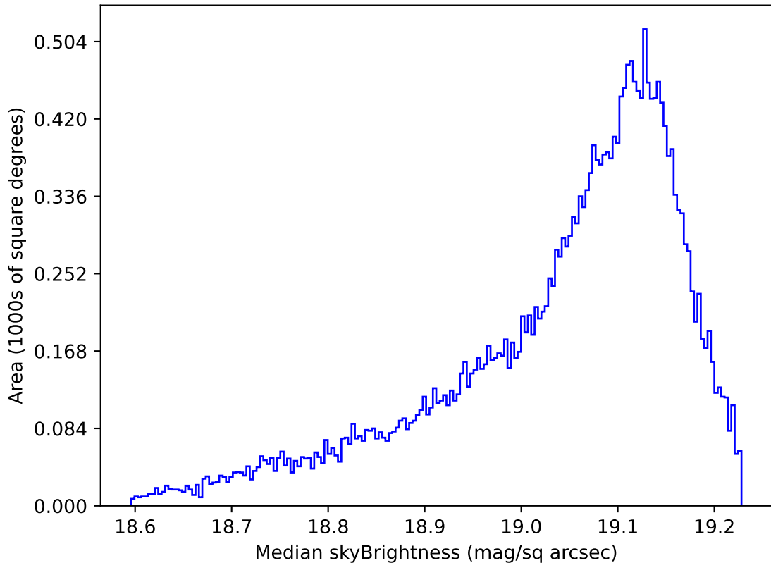
noroll_mjdp270_v3.4_10yrs All sky z band: Median skyBrightness
