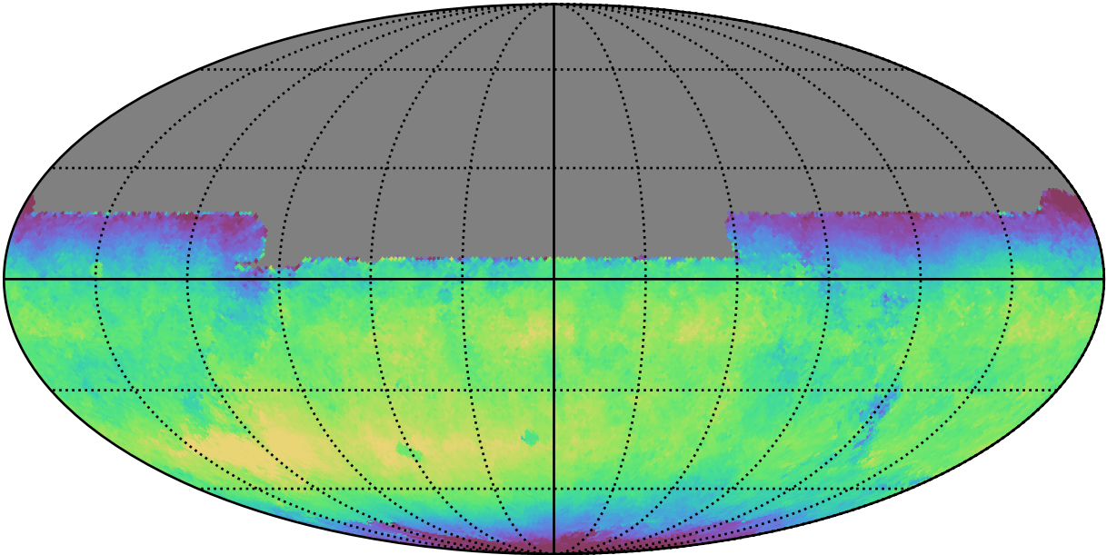
noroll_mjdp270_v3.4_10yrs All sky y band: Median skyBrightness
