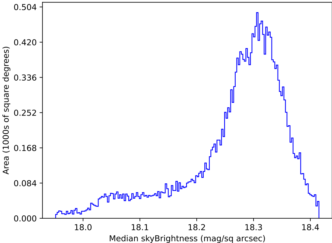
noroll_mjdp270_v3.4_10yrs All sky y band: Median skyBrightness
