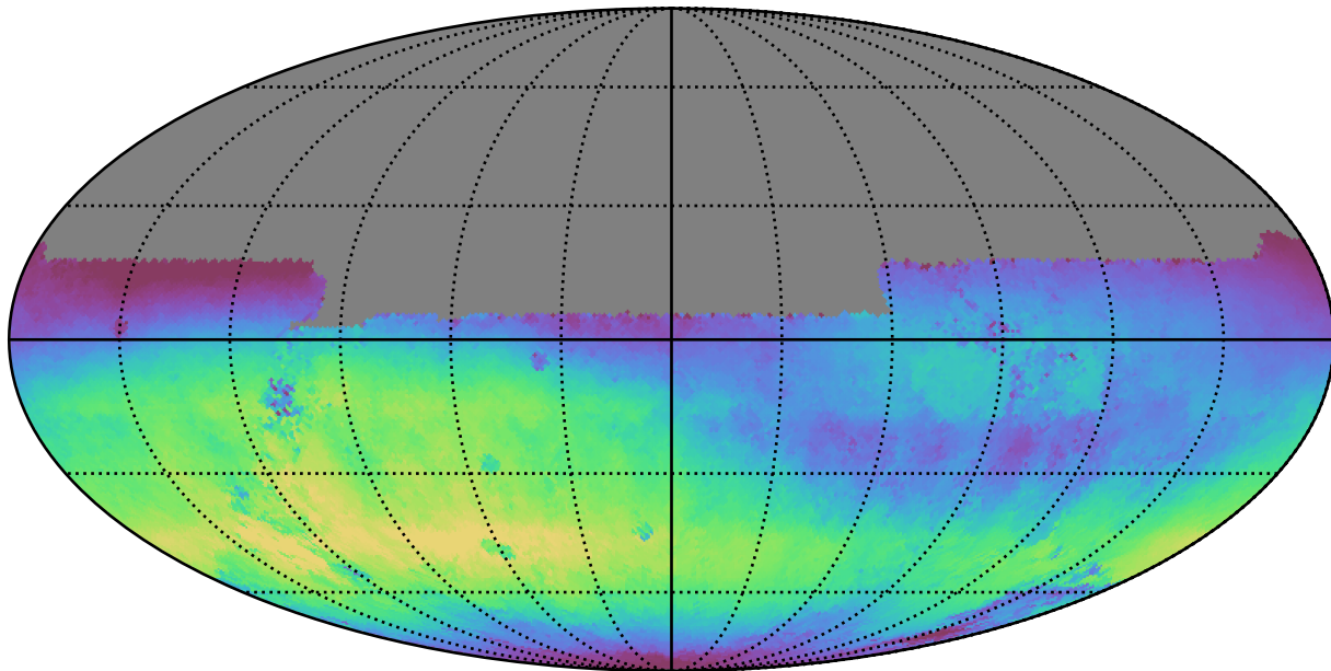
noroll_mjdp270_v3.4_10yrs All sky u band: Median skyBrightness
