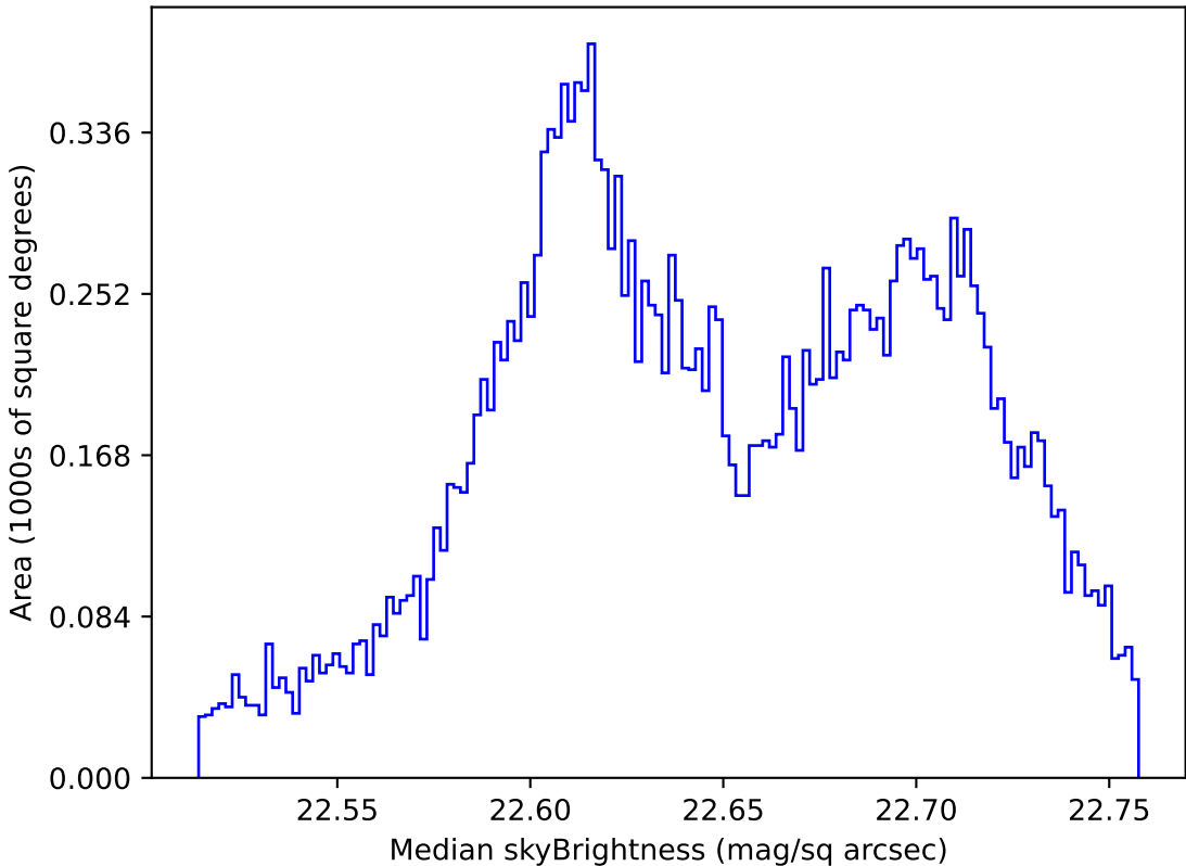
noroll_mjdp270_v3.4_10yrs All sky u band: Median skyBrightness
