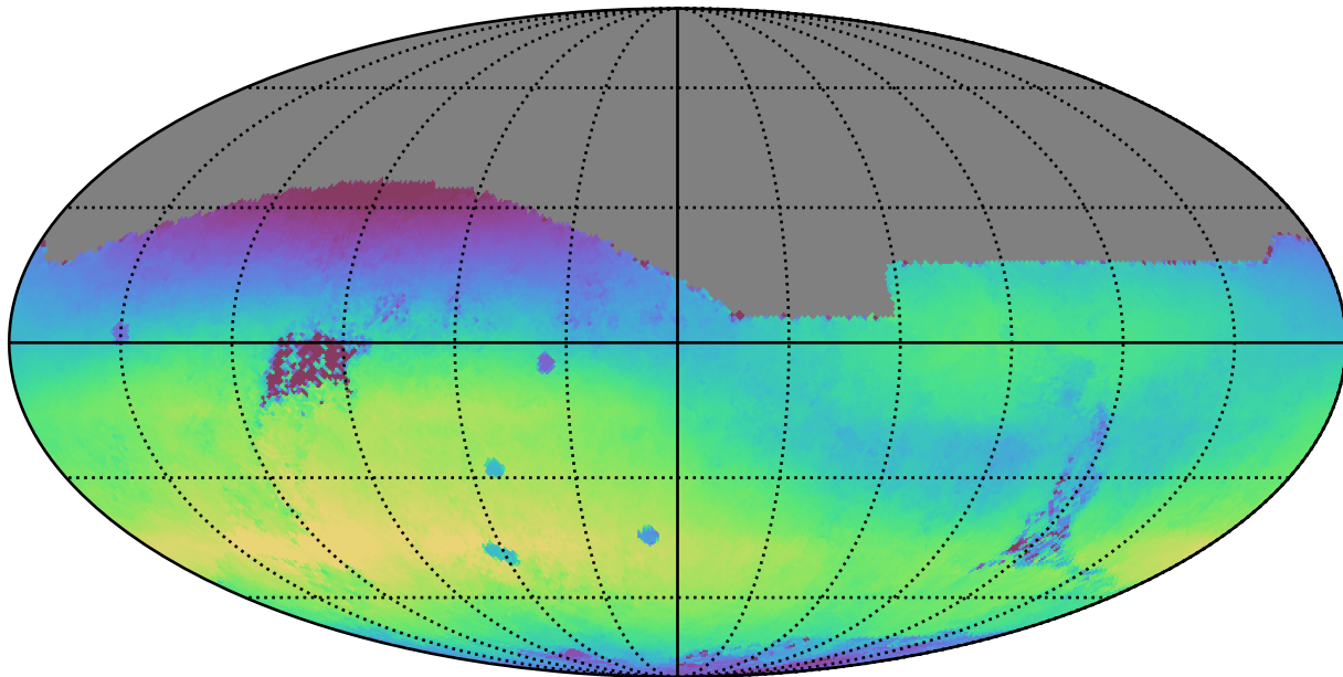
noroll_mjdp270_v3.4_10yrs All sky r band: Median skyBrightness
