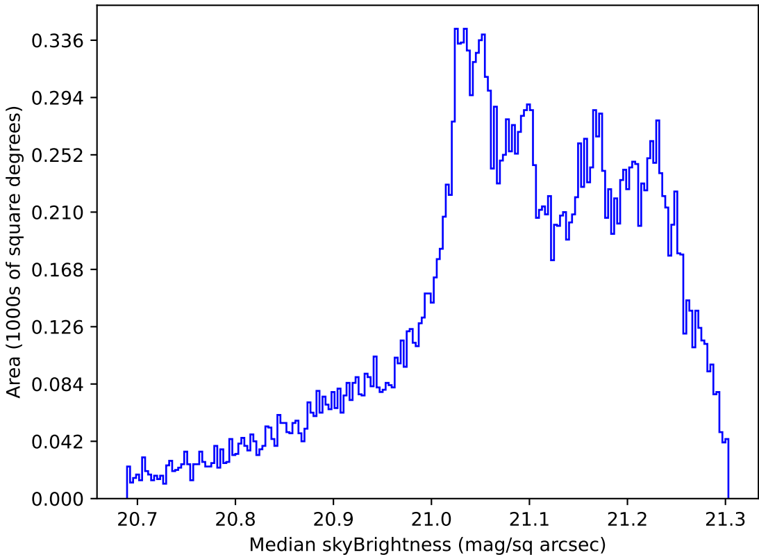
noroll_mjdp270_v3.4_10yrs All sky r band: Median skyBrightness
