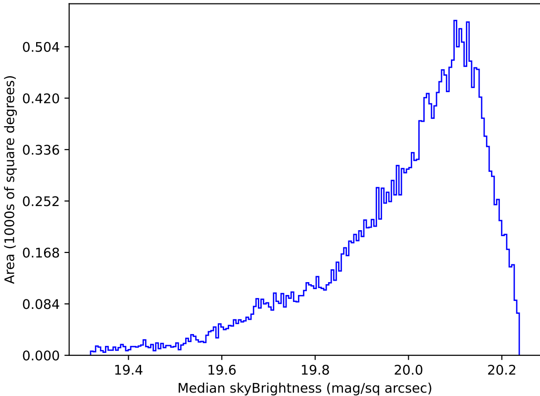
noroll_mjdp270_v3.4_10yrs All sky i band: Median skyBrightness
