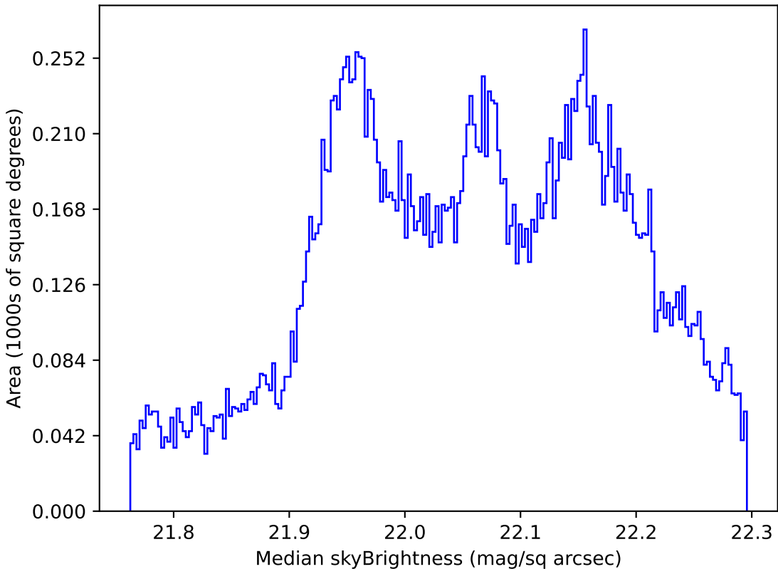
noroll_mjdp270_v3.4_10yrs All sky g band: Median skyBrightness
