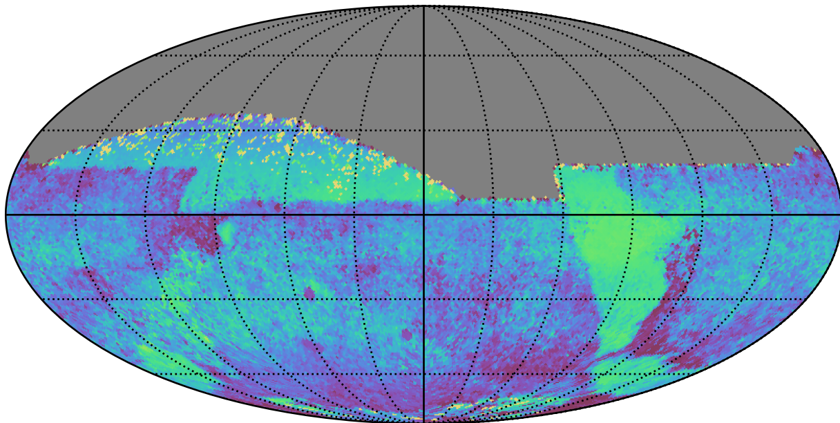
noroll_mjdp270_v3.4_10yrs All sky all bands: Median skyBrightness
