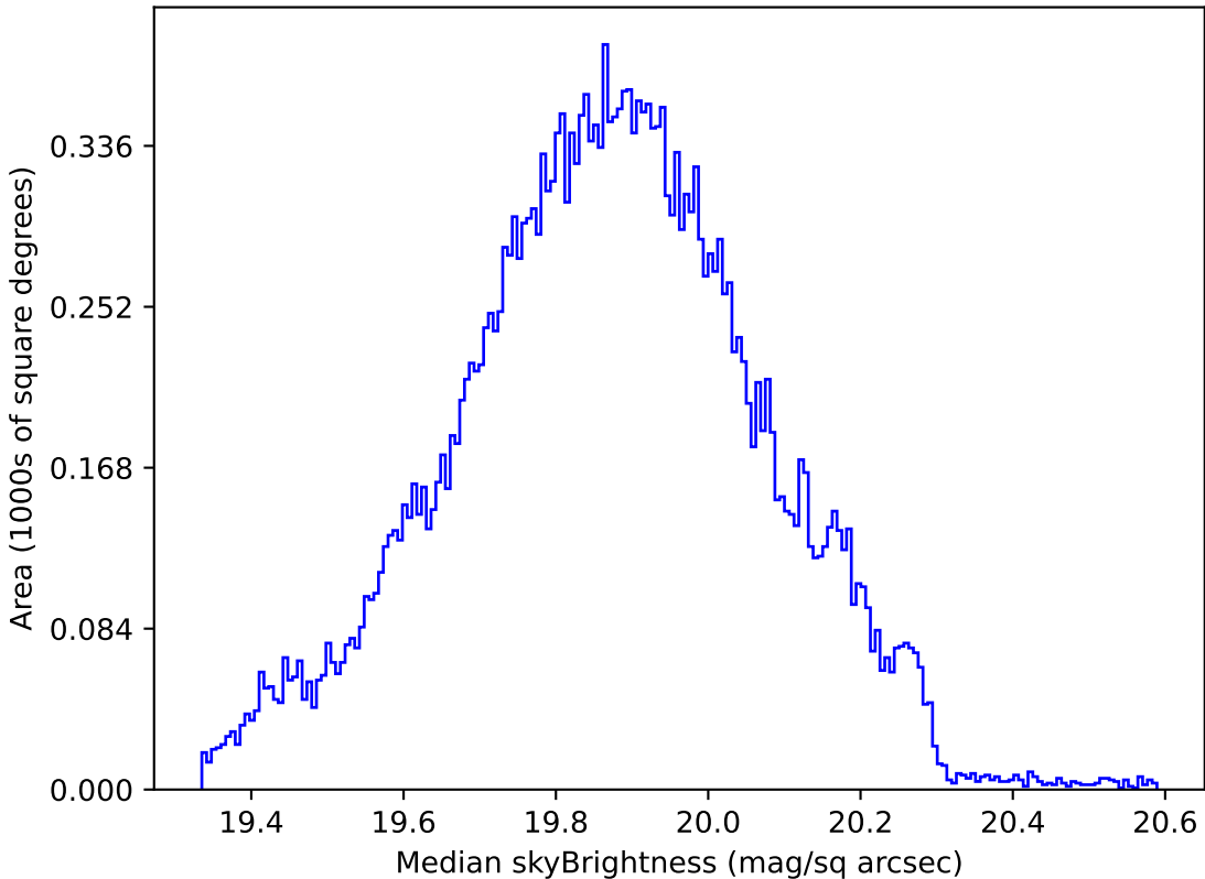
noroll_mjdp270_v3.4_10yrs All sky all bands: Median skyBrightness
