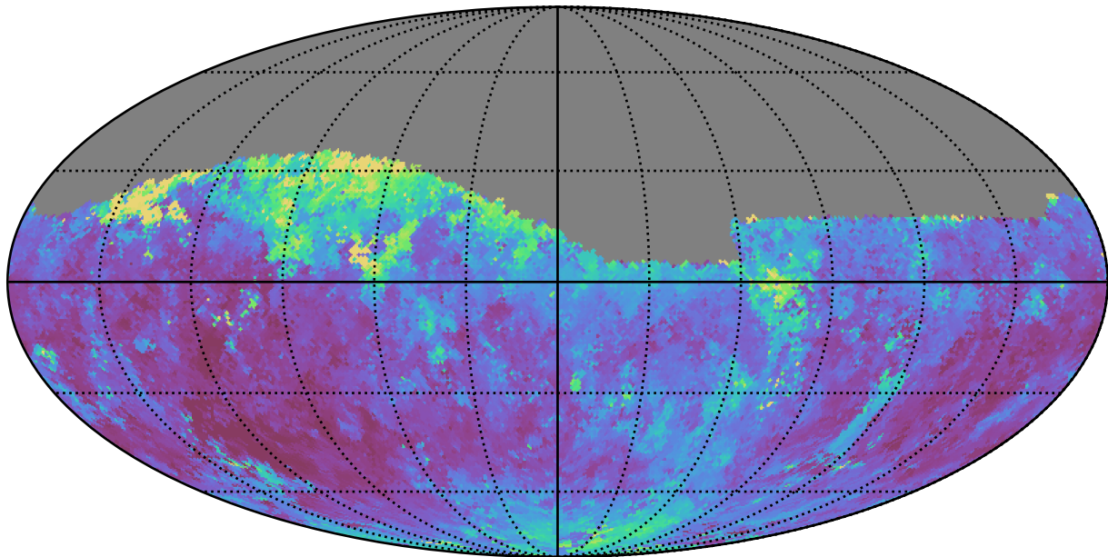
noroll_mjdp270_v3.4_10yrs Yr 1 z band: Median seeingGeom
