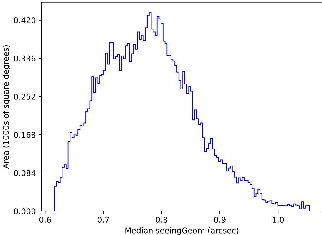
noroll_mjdp270_v3.4_10yrs Yr 1 y band: Median seeingGeom
