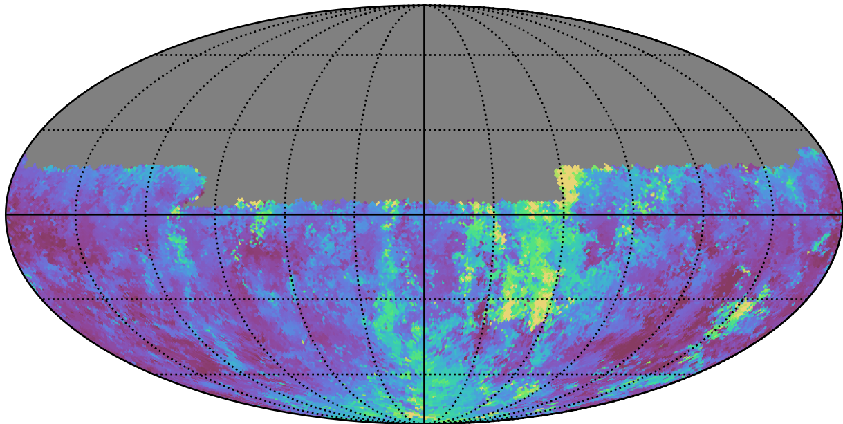
noroll_mjdp270_v3.4_10yrs Yr 1 u band: Median seeingGeom
