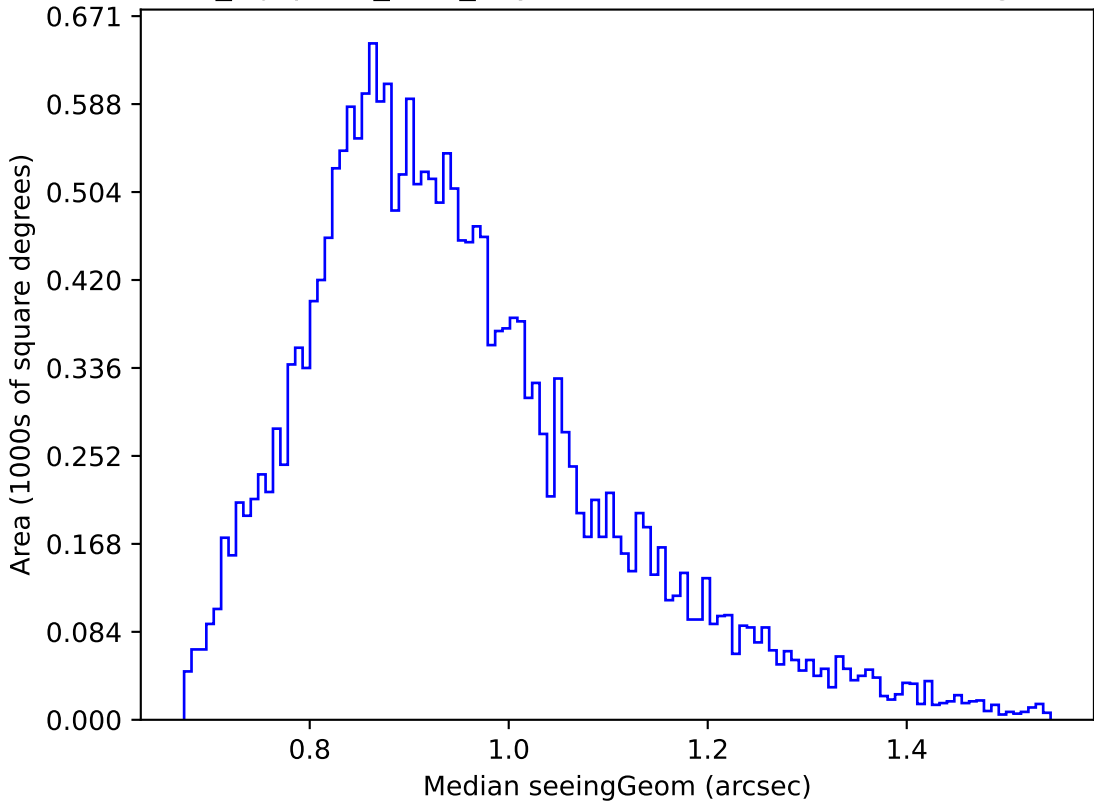
noroll_mjdp270_v3.4_10yrs Yr 1 u band: Median seeingGeom
