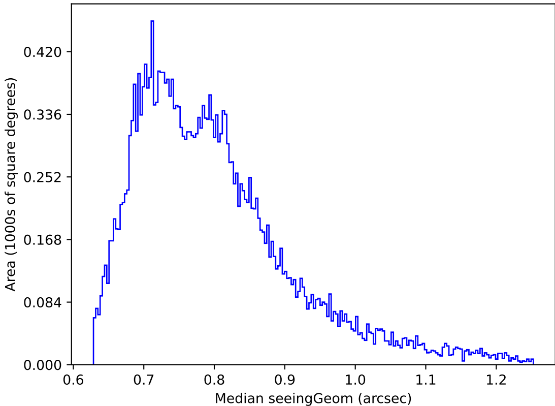
noroll_mjdp270_v3.4_10yrs Yr 1 i band: Median seeingGeom
