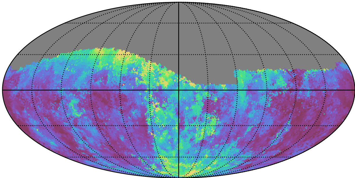
noroll_mjdp270_v3.4_10yrs Yr 1 g band: Median seeingGeom
