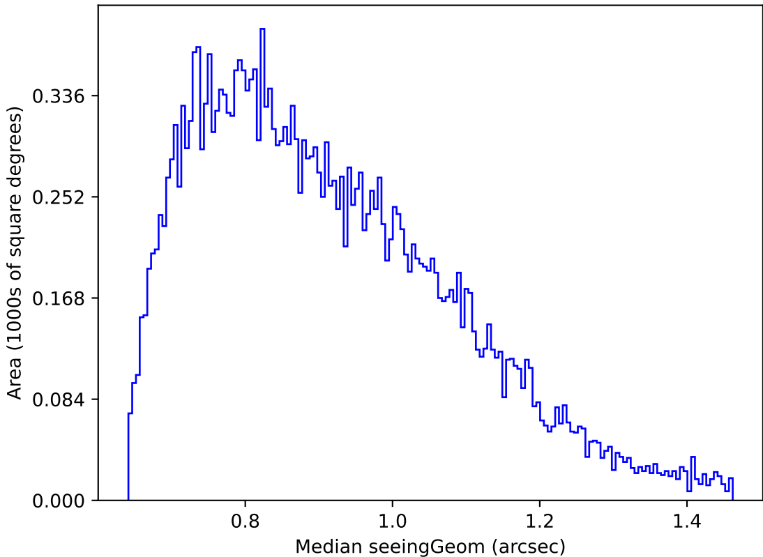
noroll_mjdp270_v3.4_10yrs Yr 1 g band: Median seeingGeom
