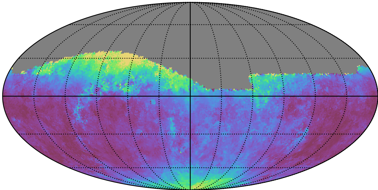
noroll_mjdp270_v3.4_10yrs Yr 1 all bands: Median seeingGeom
