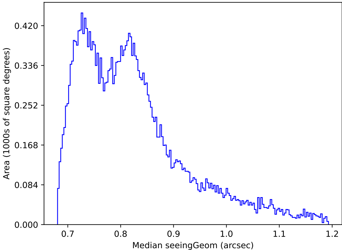
noroll_mjdp270_v3.4_10yrs Yr 1 all bands: Median seeingGeom
