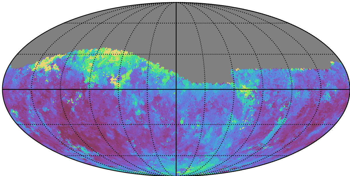
noroll_mjdp270_v3.4_10yrs Yr 1 z band: Median seeingEff
