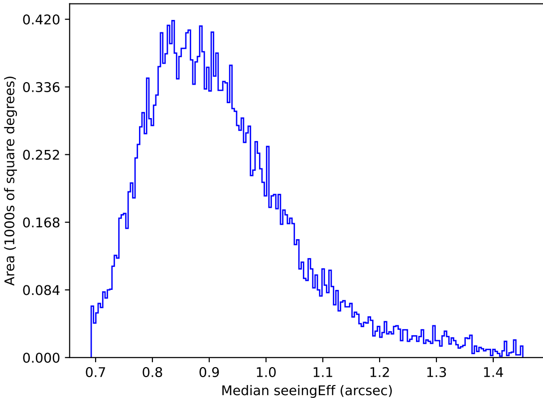
noroll_mjdp270_v3.4_10yrs Yr 1 z band: Median seeingEff
