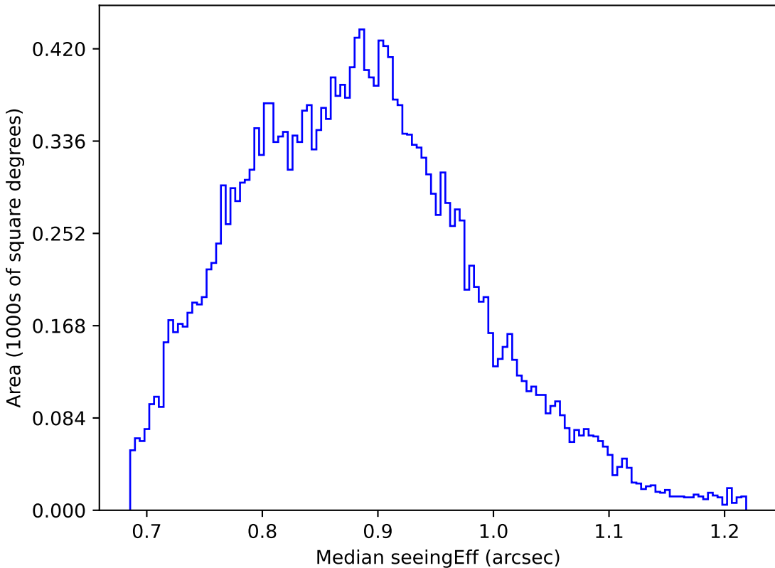
noroll_mjdp270_v3.4_10yrs Yr 1 y band: Median seeingEff
