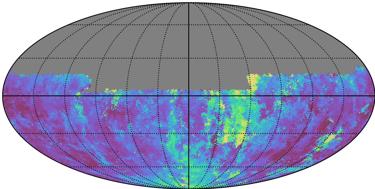
noroll_mjdp270_v3.4_10yrs Yr 1 u band: Median seeingEff
