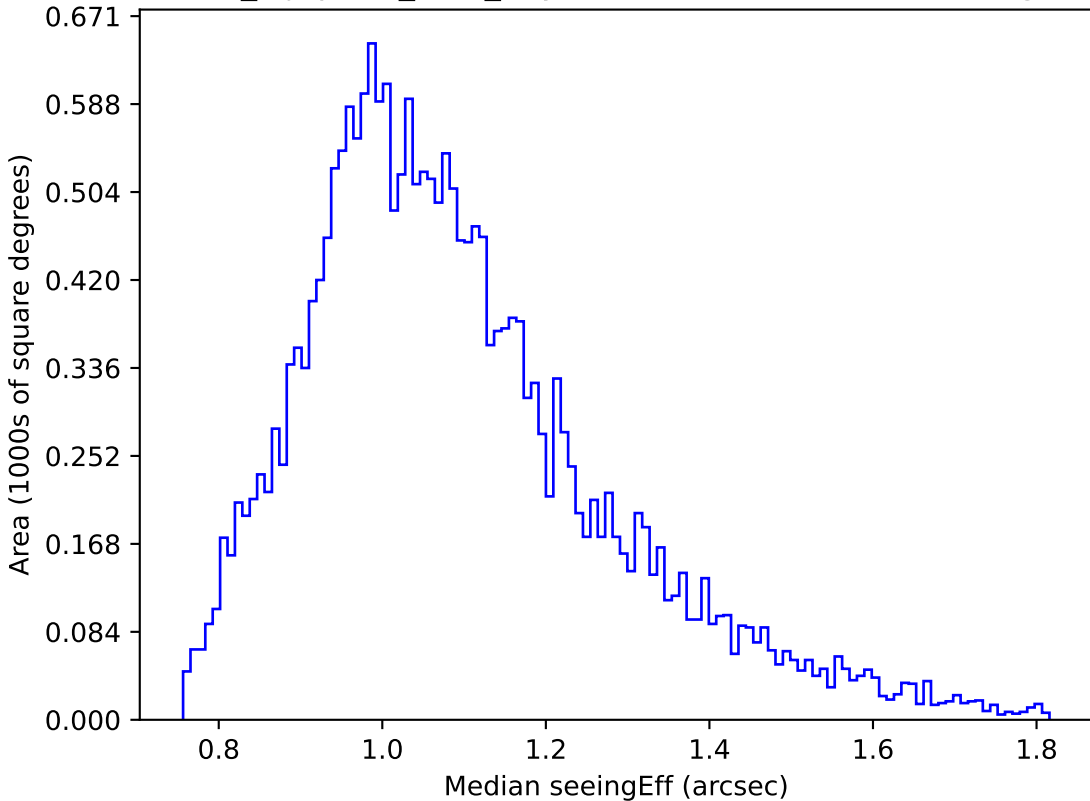
noroll_mjdp270_v3.4_10yrs Yr 1 u band: Median seeingEff
