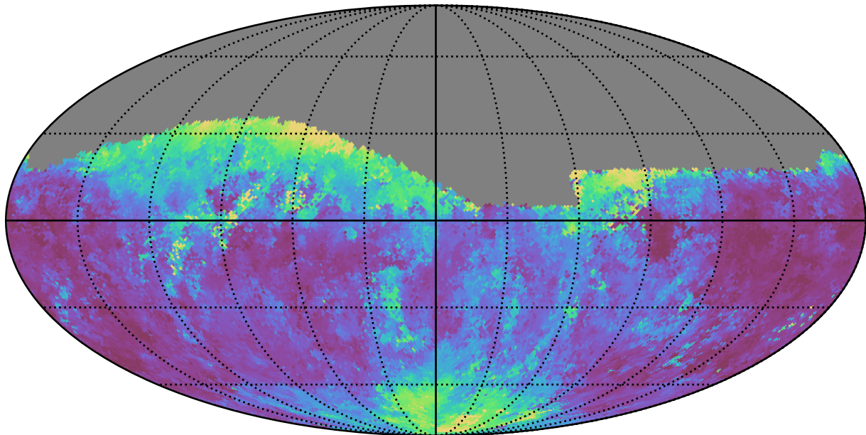
noroll_mjdp270_v3.4_10yrs Yr 1 r band: Median seeingEff
