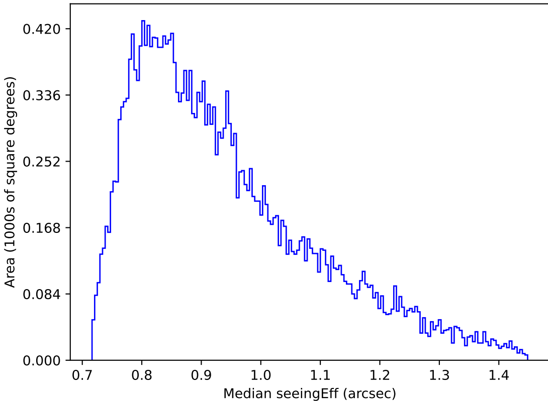
noroll_mjdp270_v3.4_10yrs Yr 1 r band: Median seeingEff
