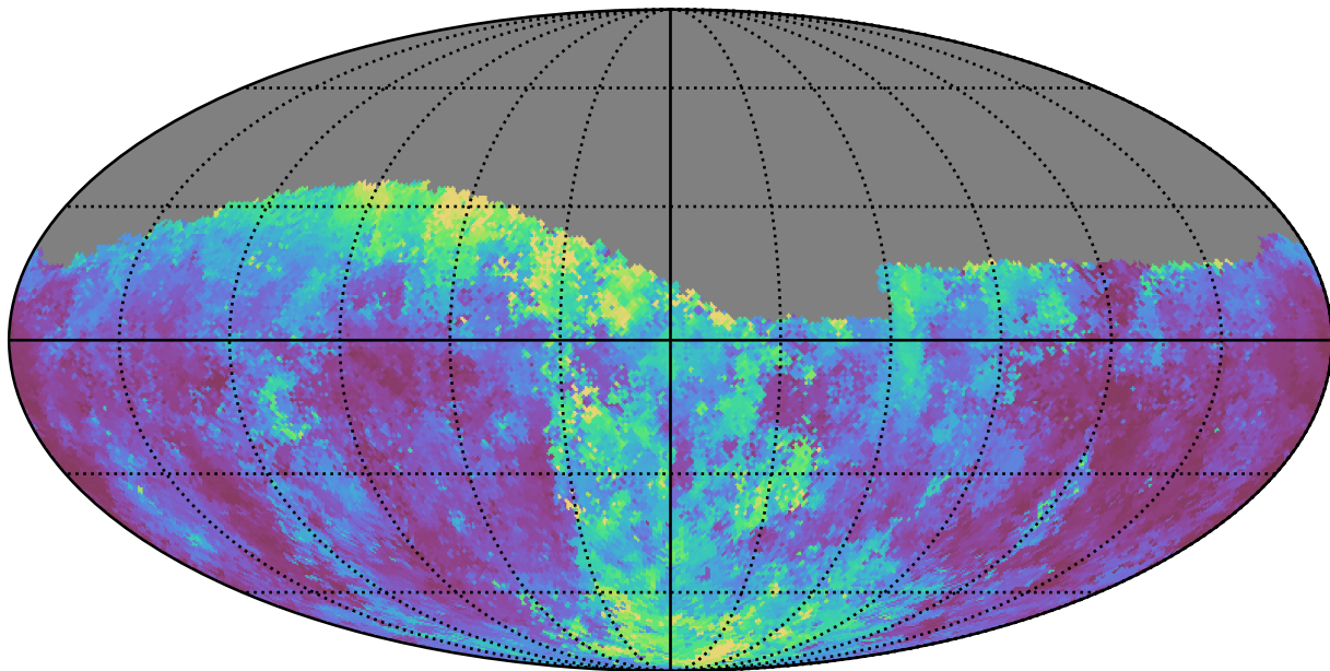
noroll_mjdp270_v3.4_10yrs Yr 1 g band: Median seeingEff
