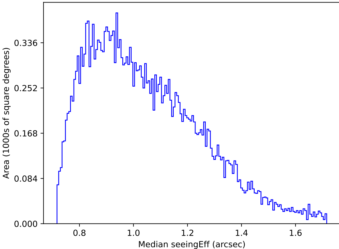
noroll_mjdp270_v3.4_10yrs Yr 1 g band: Median seeingEff
