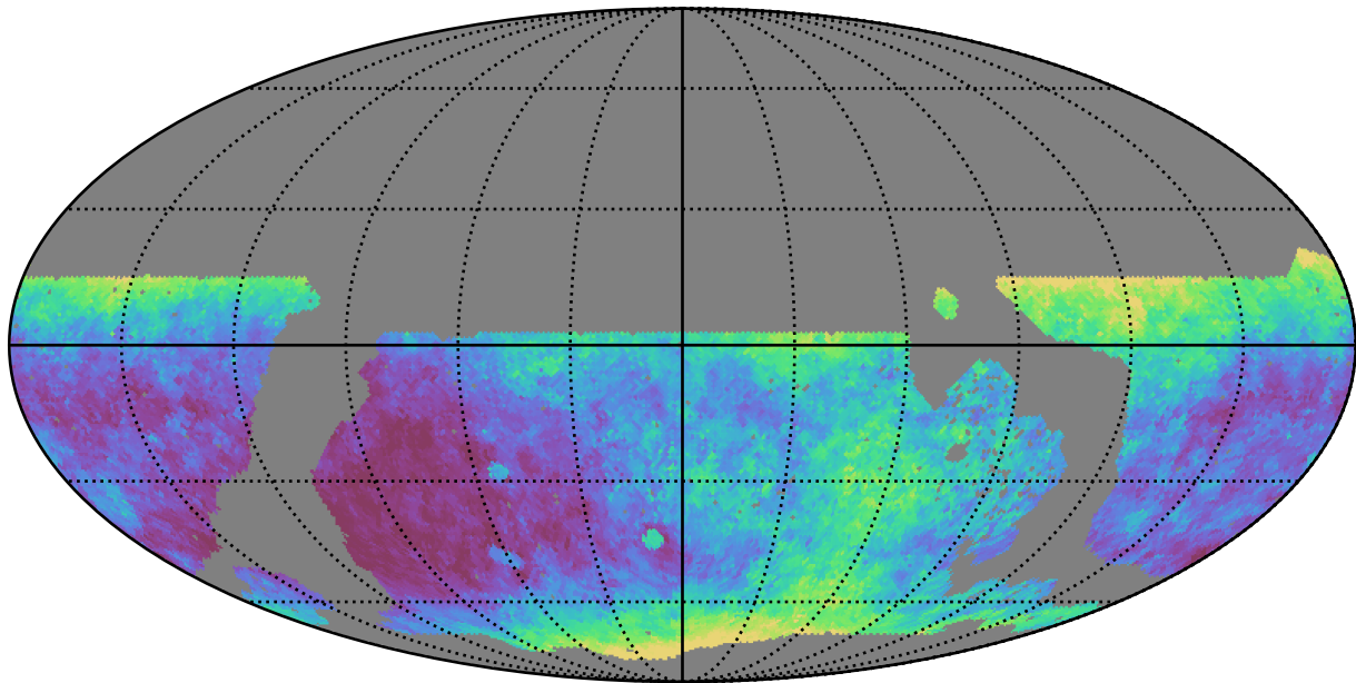
noroll_mjdp270_v3.4_10yrs WFD z band: Median seeingEff
