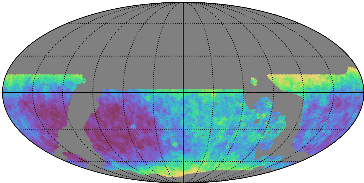
noroll_mjdp270_v3.4_10yrs WFD y band: Median seeingEff
