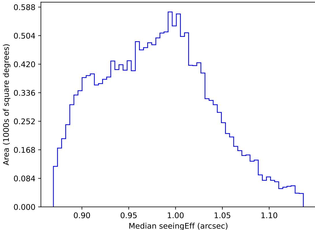
noroll_mjdp270_v3.4_10yrs WFD y band: Median seeingEff
