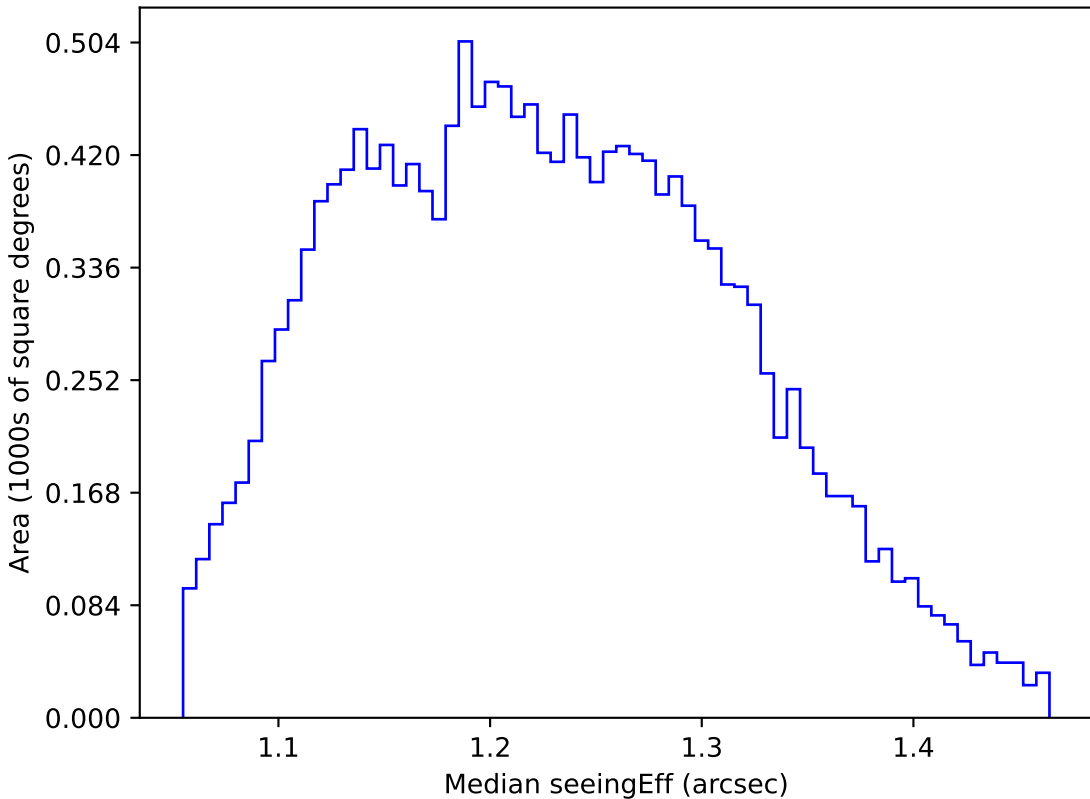
noroll_mjdp270_v3.4_10yrs WFD u band: Median seeingEff
