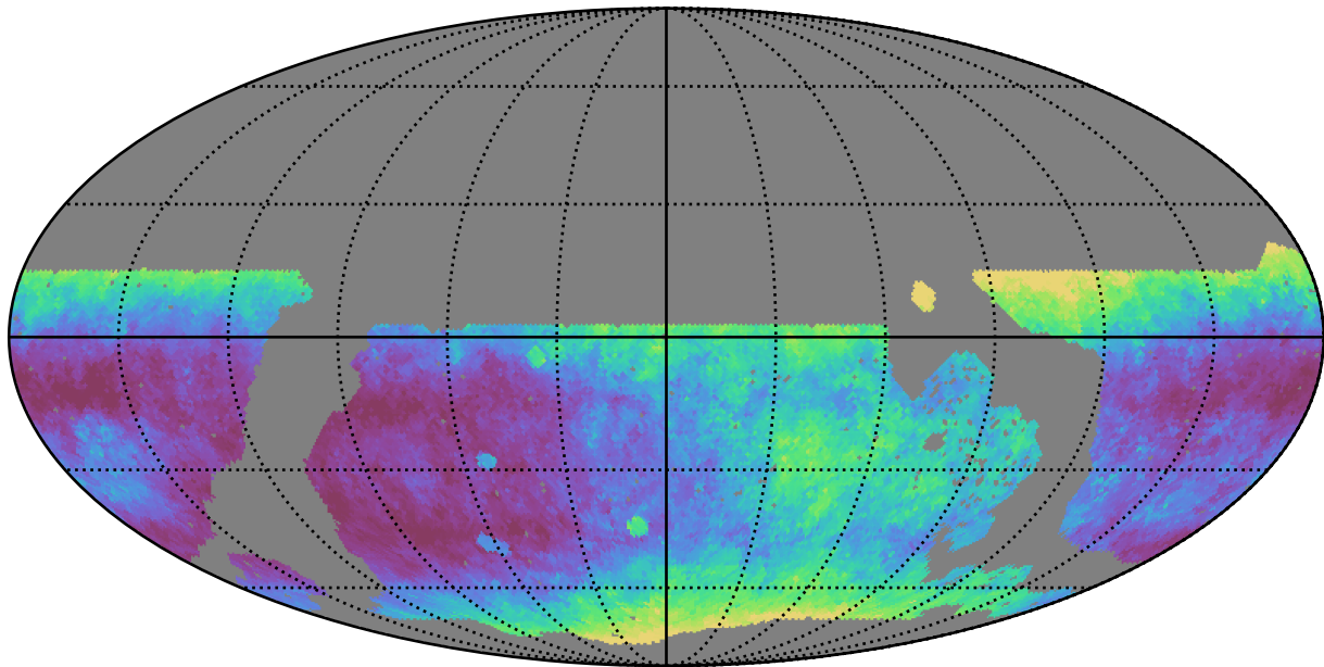
noroll_mjdp270_v3.4_10yrs WFD r band: Median seeingEff
