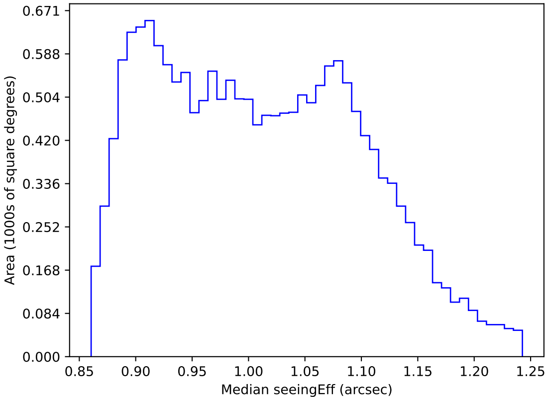
noroll_mjdp270_v3.4_10yrs WFD r band: Median seeingEff
