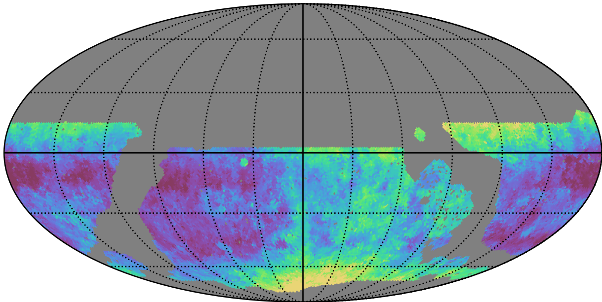
noroll_mjdp270_v3.4_10yrs WFD g band: Median seeingEff
