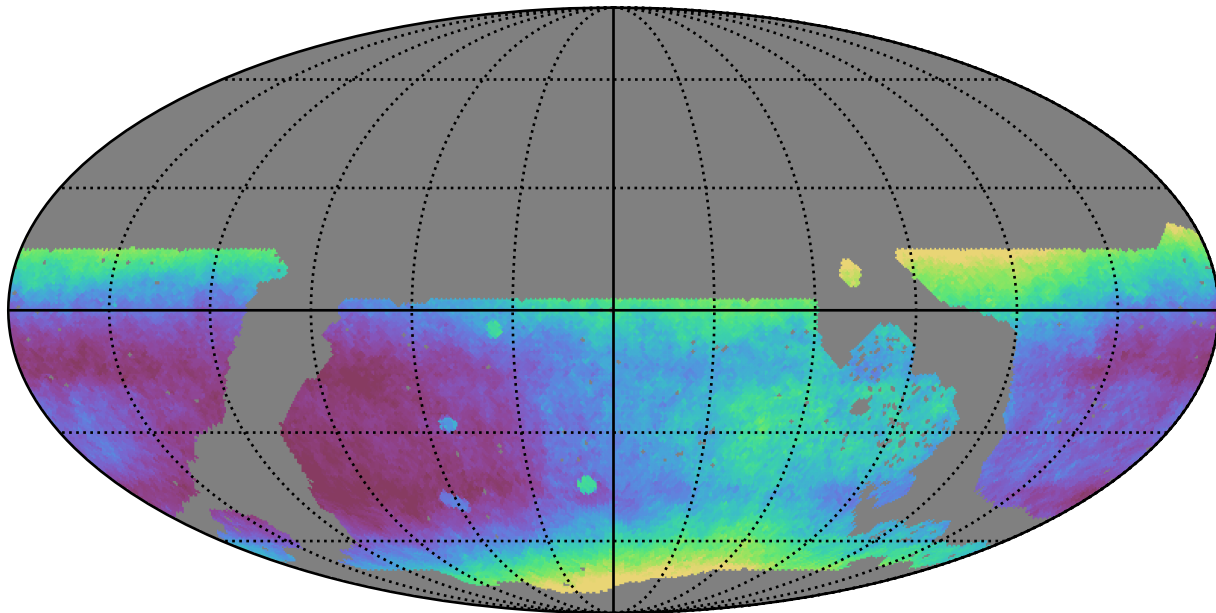
noroll_mjdp270_v3.4_10yrs WFD all bands: Median seeingEff
