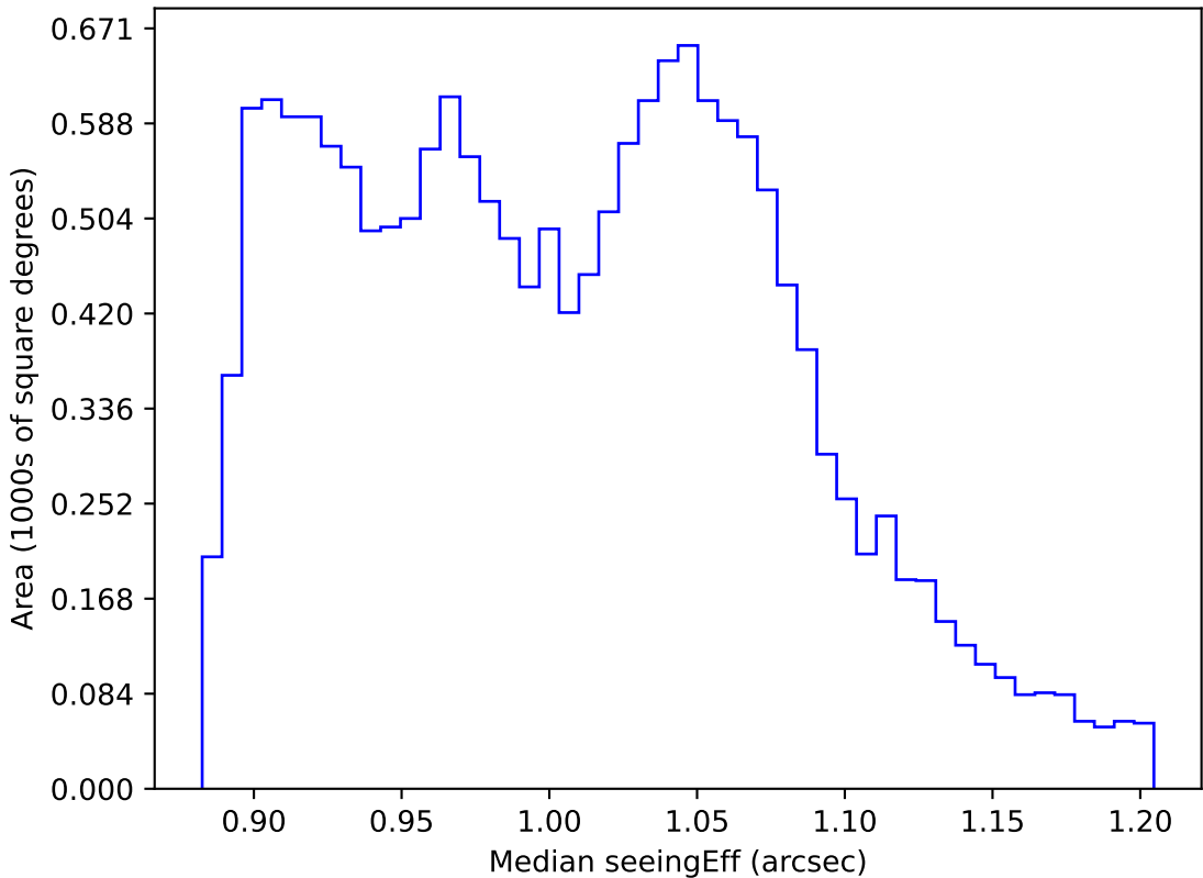
noroll_mjdp270_v3.4_10yrs WFD all bands: Median seeingEff
